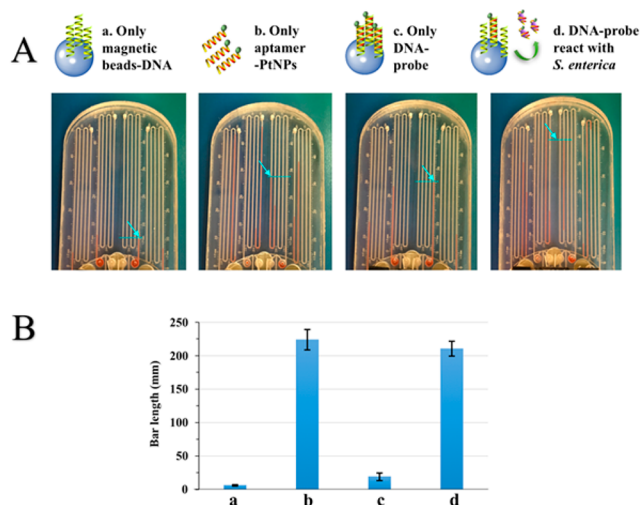
Figure 3. Photograph (A) and corresponding histogram of visual bar-chart (B) at different conditions: (a) only magnetic beads–DNA, (b) only PtNPs–aptamer, (c) only DNA probe, and (d) DNA probe reacting with S. enterica . The blue arrows and dotted lines indicate the end point of the dye bar and the quantitative values of scale marker, respectively. The standard deviation was obtained from four parallel measurements.
